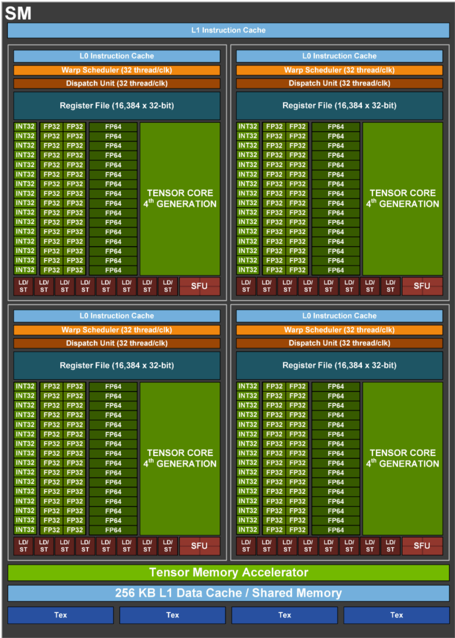
Figure 4. GH100 streaming multiprocessor
