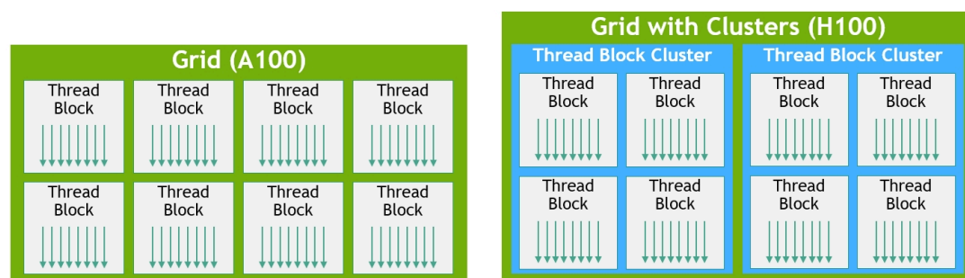
Figure 11. Thread block clusters and grids with clusters
