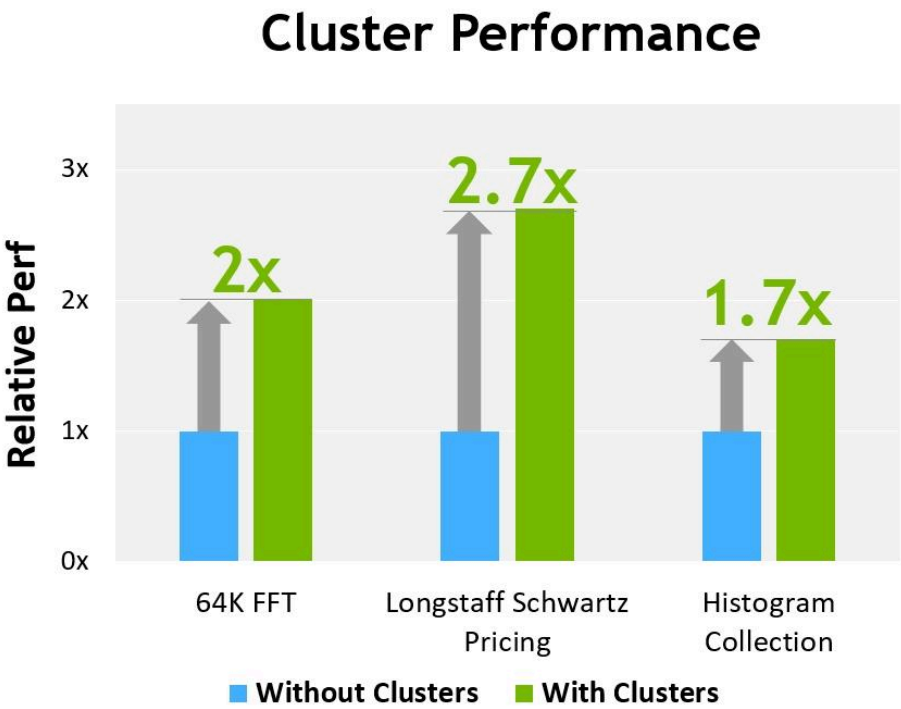
Figure 13. Cluster vs. non-cluster performance comparisons
