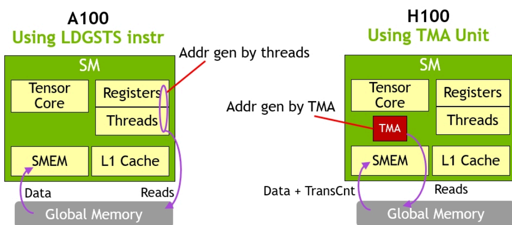
Figure 16. Asynchronous memory copy with TMA on H100 vs. LDGSTS on A100
