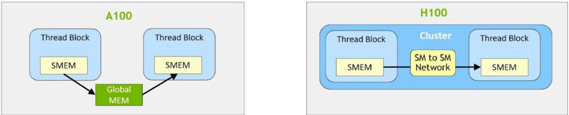
Figure 12. Thread-block-to-thread-block data exchange (A100 vs. H100 with clusters)
