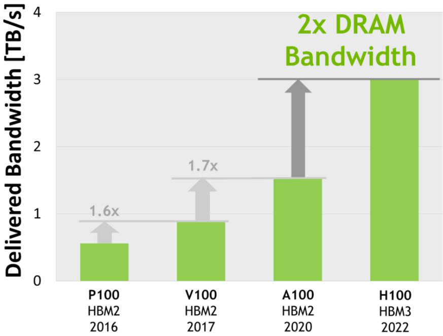
Figure 18. World’s first HBM3 GPU memory architecture, 2x delivered bandwidth
